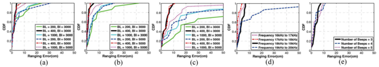
Fig. 6. Beep design: results obtained from HTC EVO. (a) BL and BI design, 100cm. (b) BL and BI design, 200cm. (c) BL and BI design, 300cm. (d) Frequency design, 300cm. (e) Number of beeps design, 300cm.
